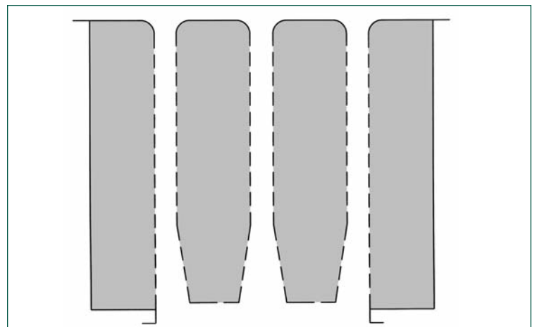
Schematic of splitter design shows external half splitters (EX model).
