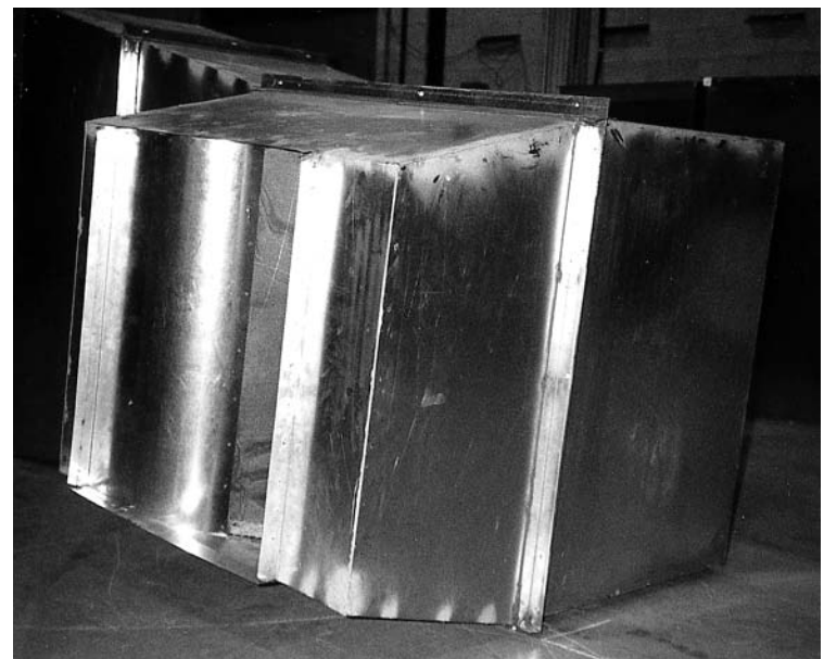
Photo of elbow transitional silencer on its side ready for test. Connection (to AH unit) size is less than external cross sectional body size (ex-type for lower pressure drop).
